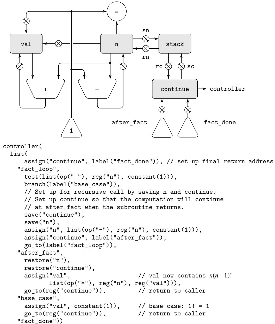
Figure 5.11 A recursive factorial machine.
