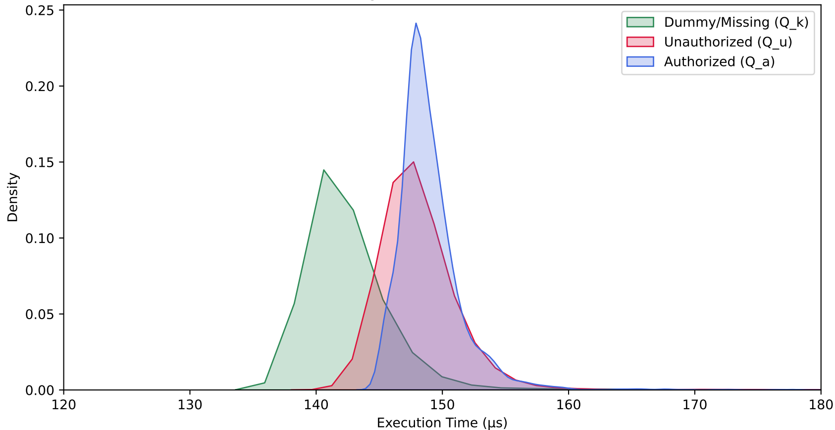
RLS Timing Side-Channel (All 3 States)
