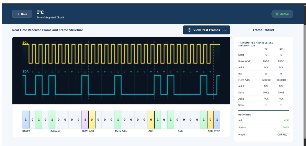
Figure 5.6: I2C frame for CORRECT case
