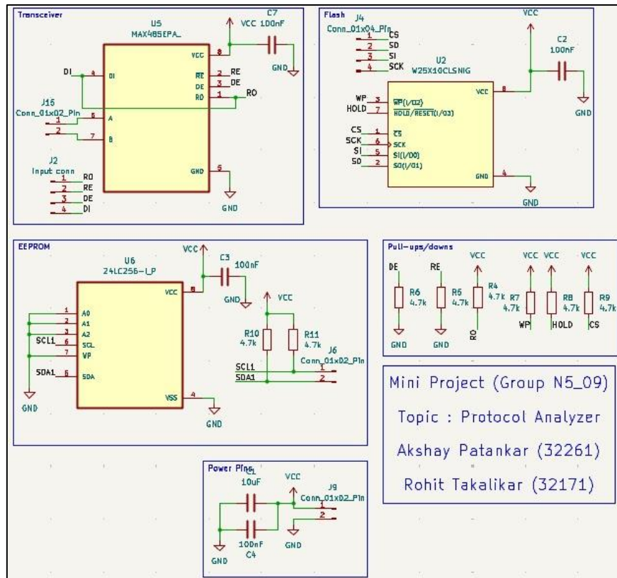
Figure 4.4.2: Final Schematic
