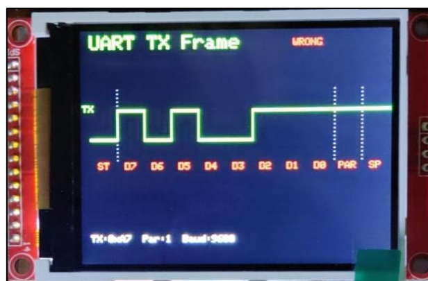
Figure 5.5.1: UART transmitted frame for WRONG case
