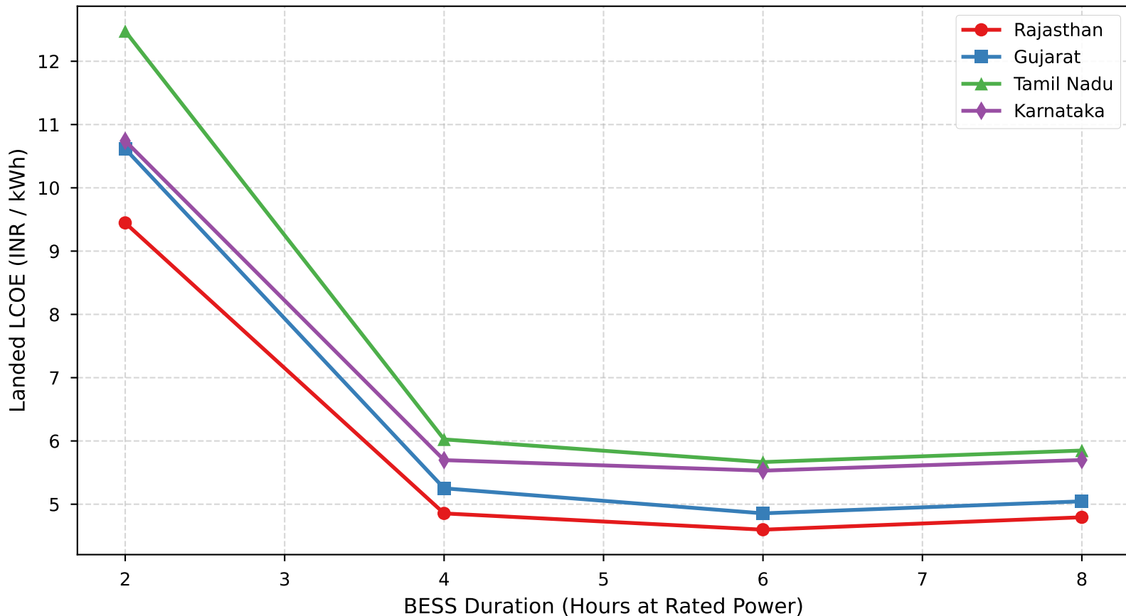
Landed LCOE Sensitivity to Battery Storage Duration (FY 2029-30, 43.3% RPO Mandate)
