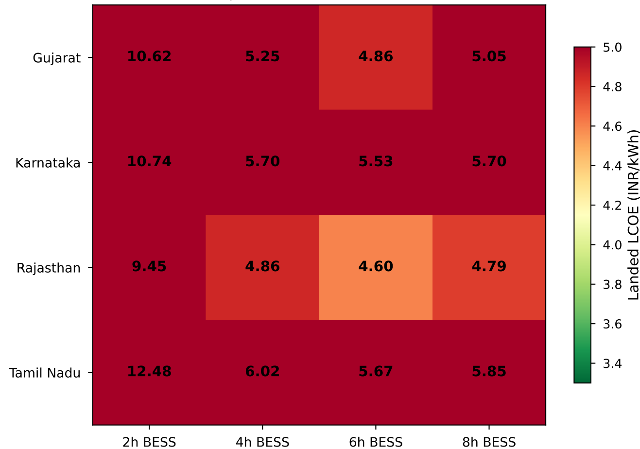
(b) FY 2029-30 Landed LCOE Heatmap (INR/kWh) by State and BESS Duration
