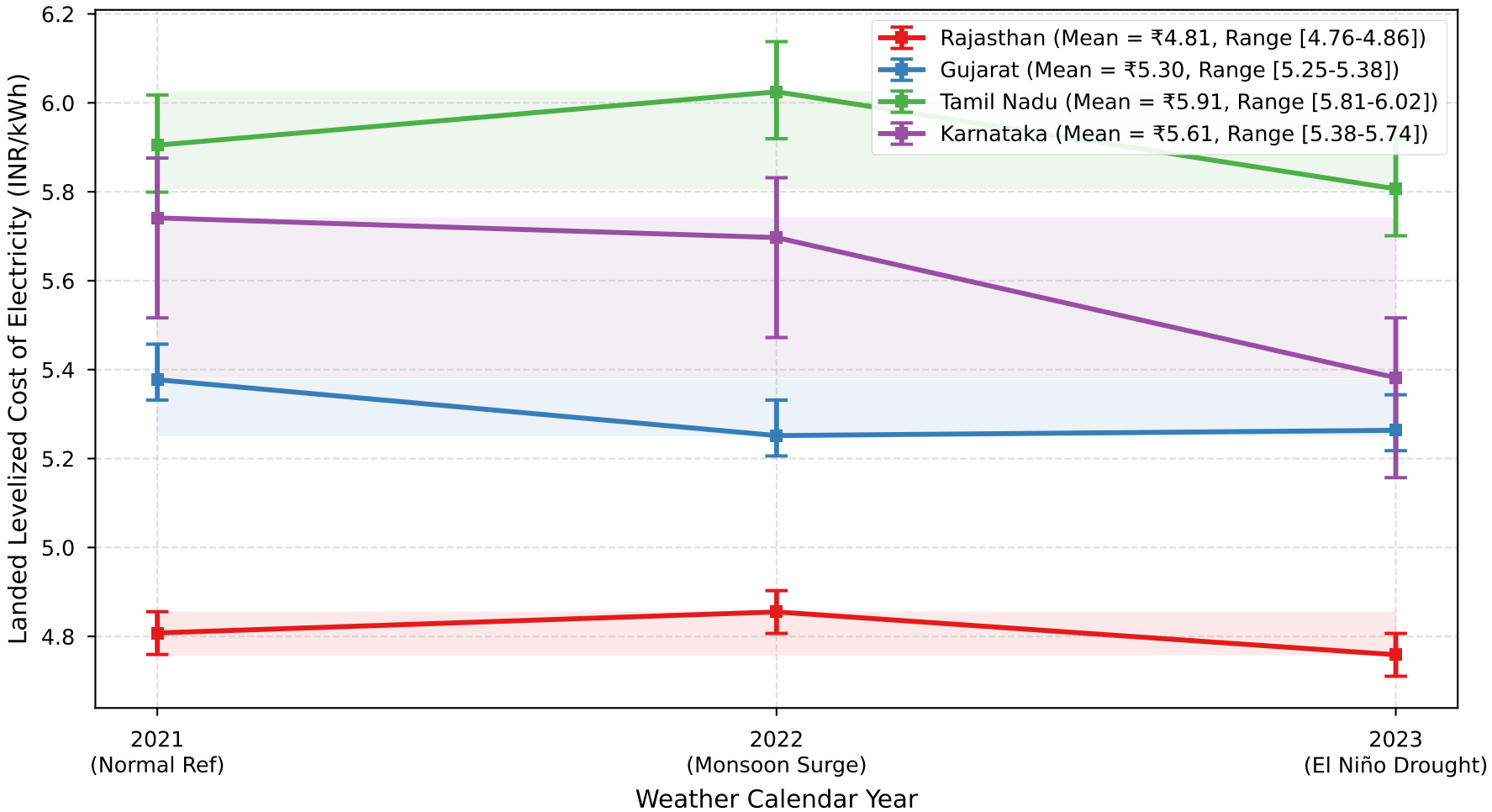
Inter-Annual Landed LCOE Robustness Across 3 Historical Weather Calendar Years (FY 2029-30, 4h BESS)
