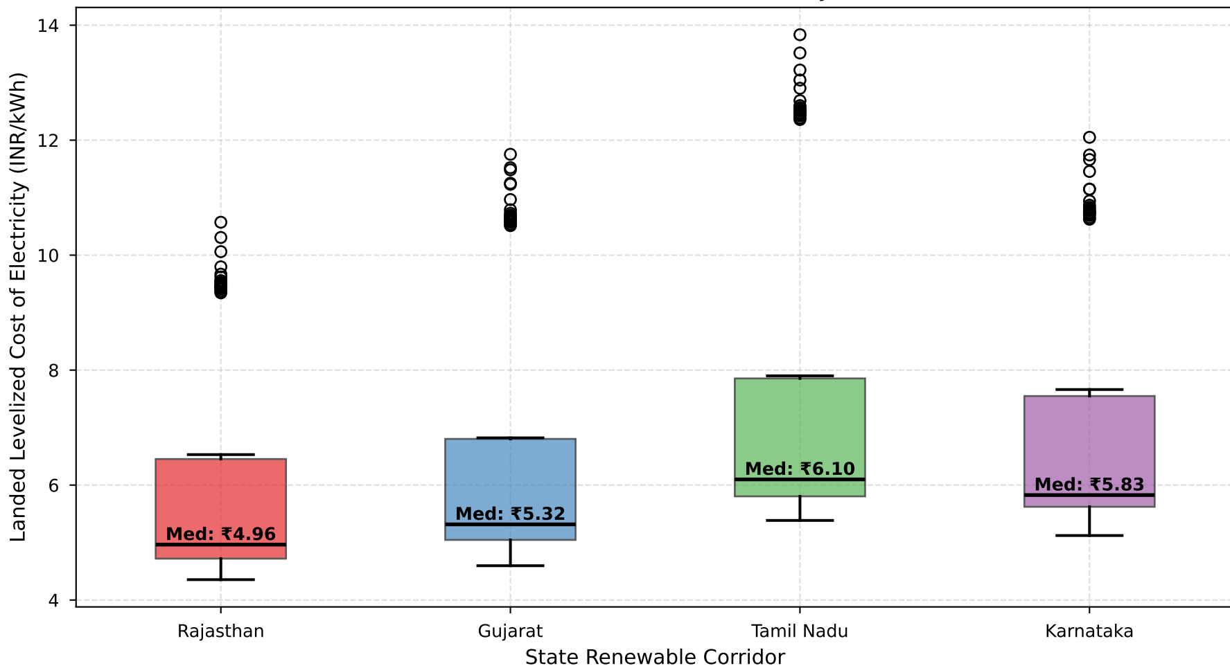
Landed LCOE Distribution Across All 288 Solved Policy & Technical Scenarios
