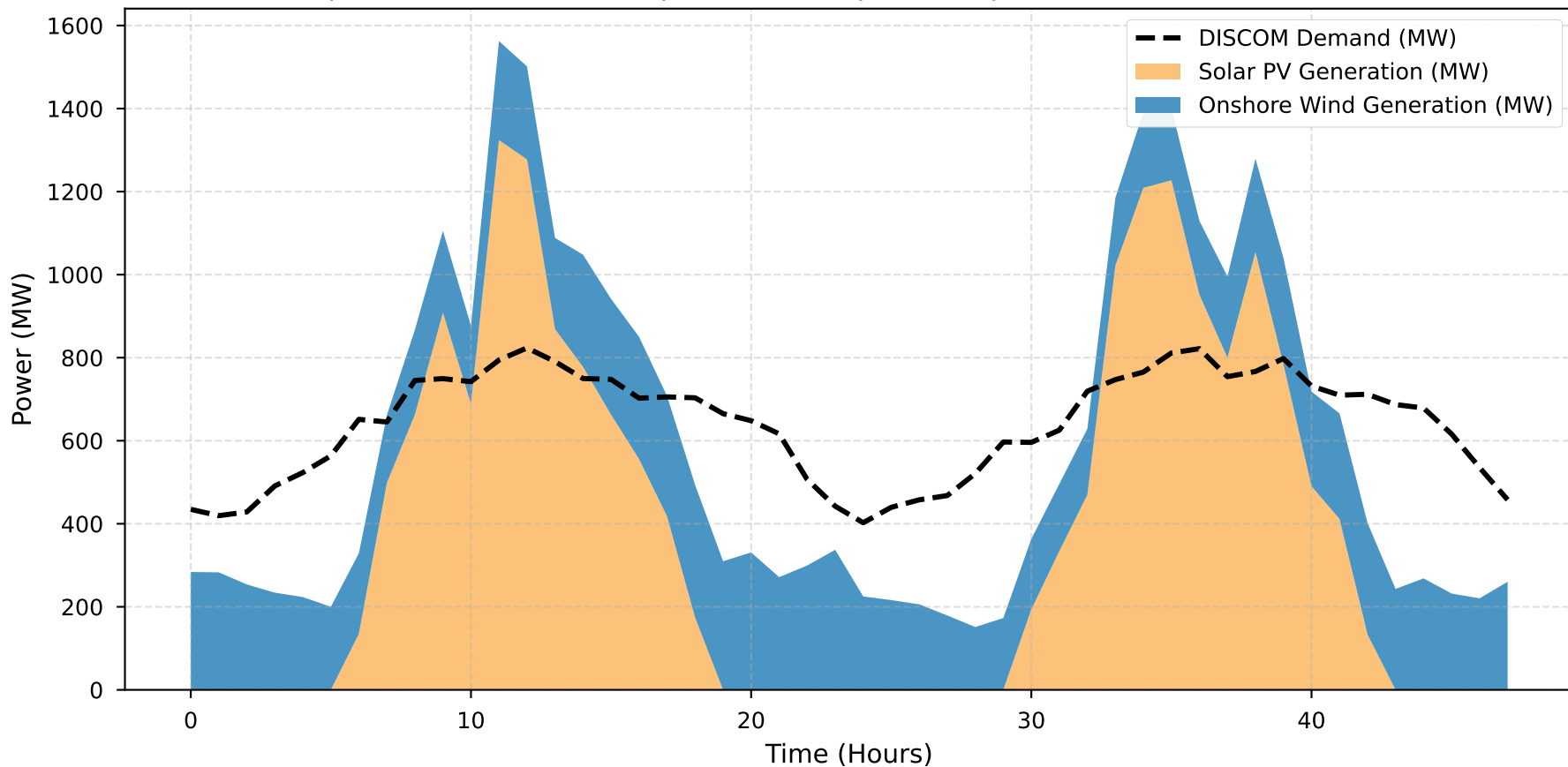
Representative 48-Hour Operational Dispatch (Rajasthan FY 2029-30 Baseline)
