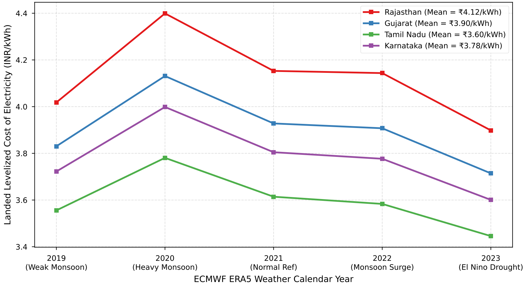
Inter-Annual Landed LCOE Robustness Across 5 Historical ERA5 Weather Reanalysis Years (FY 2029-30, 4h BESS)
