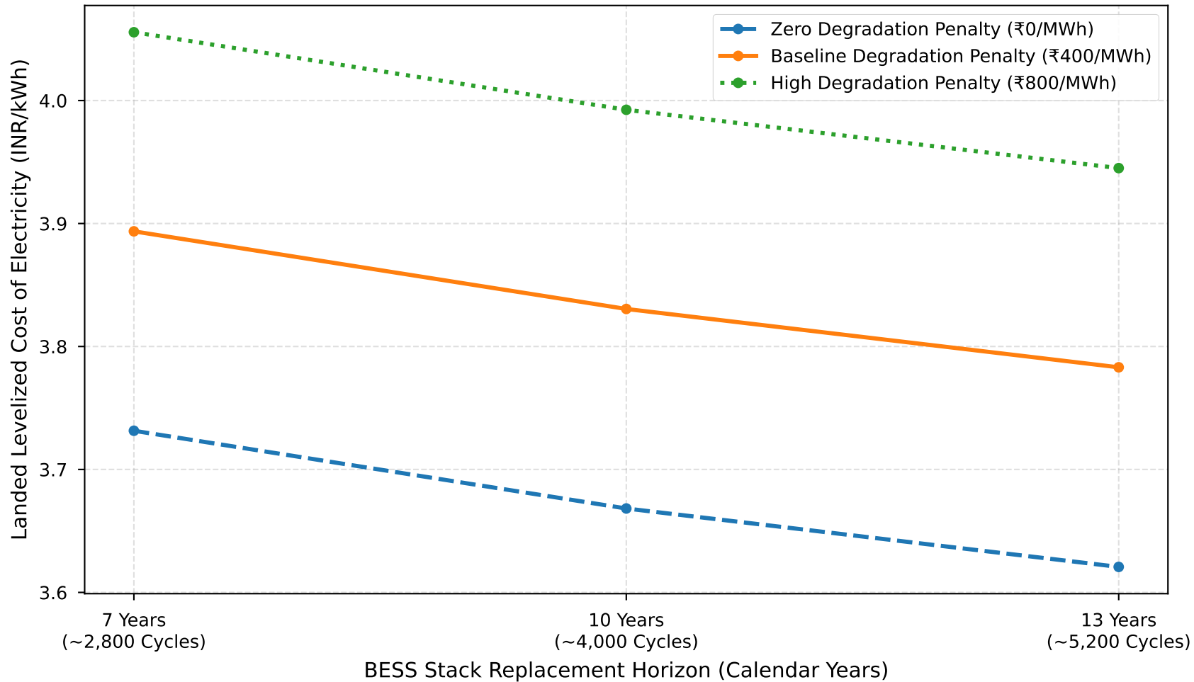
Landed LCOE Sensitivity to BESS Cell Stack Replacement Lifespan & Wear Penalties (Rajasthan 2029-30)
