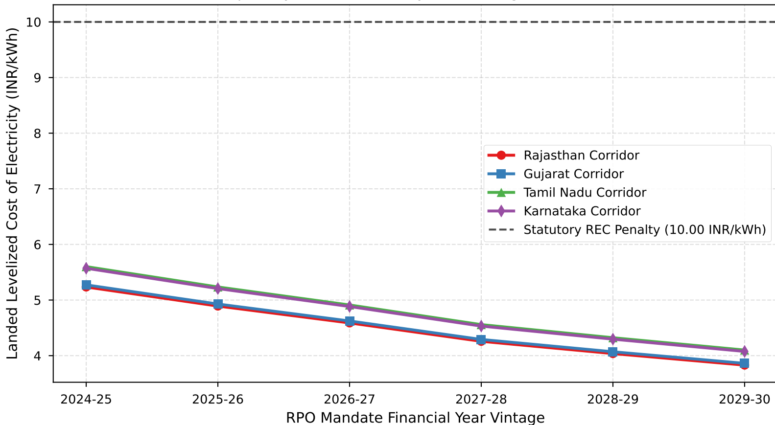
Landed LCOE Trajectory across Statutory RPO Vintages (4-Hour BESS Baseline)
