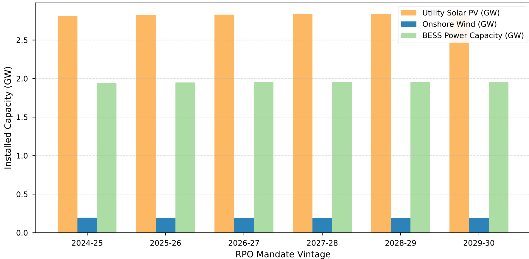
Optimal Hybrid Capacity Build-out for 1,000 MW Peak DISCOM Load (Rajasthan Corridor)
