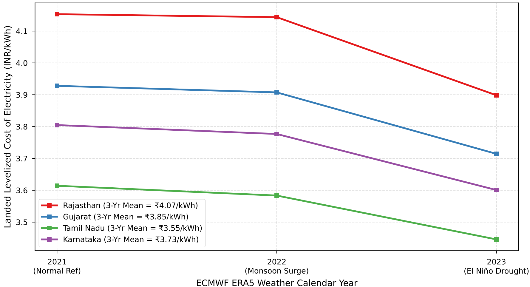
Inter-Annual Landed LCOE Robustness Across 3 Historical ERA5 Weather Reanalysis Years (FY 2029-30, 4h BESS)
