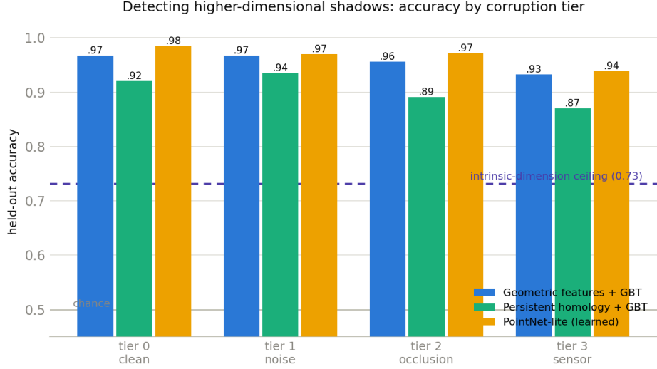
Figure 4: Accuracy by corruption tier. Both feature-based and learned methods sit far above the intrinsic-dimension ceiling (dashed) at every tier and degrade gracefully under noise, occlusion, and sensor-like dropout.
