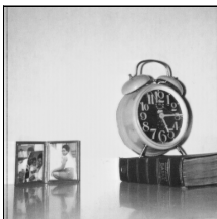
Noise (d=0.07)
