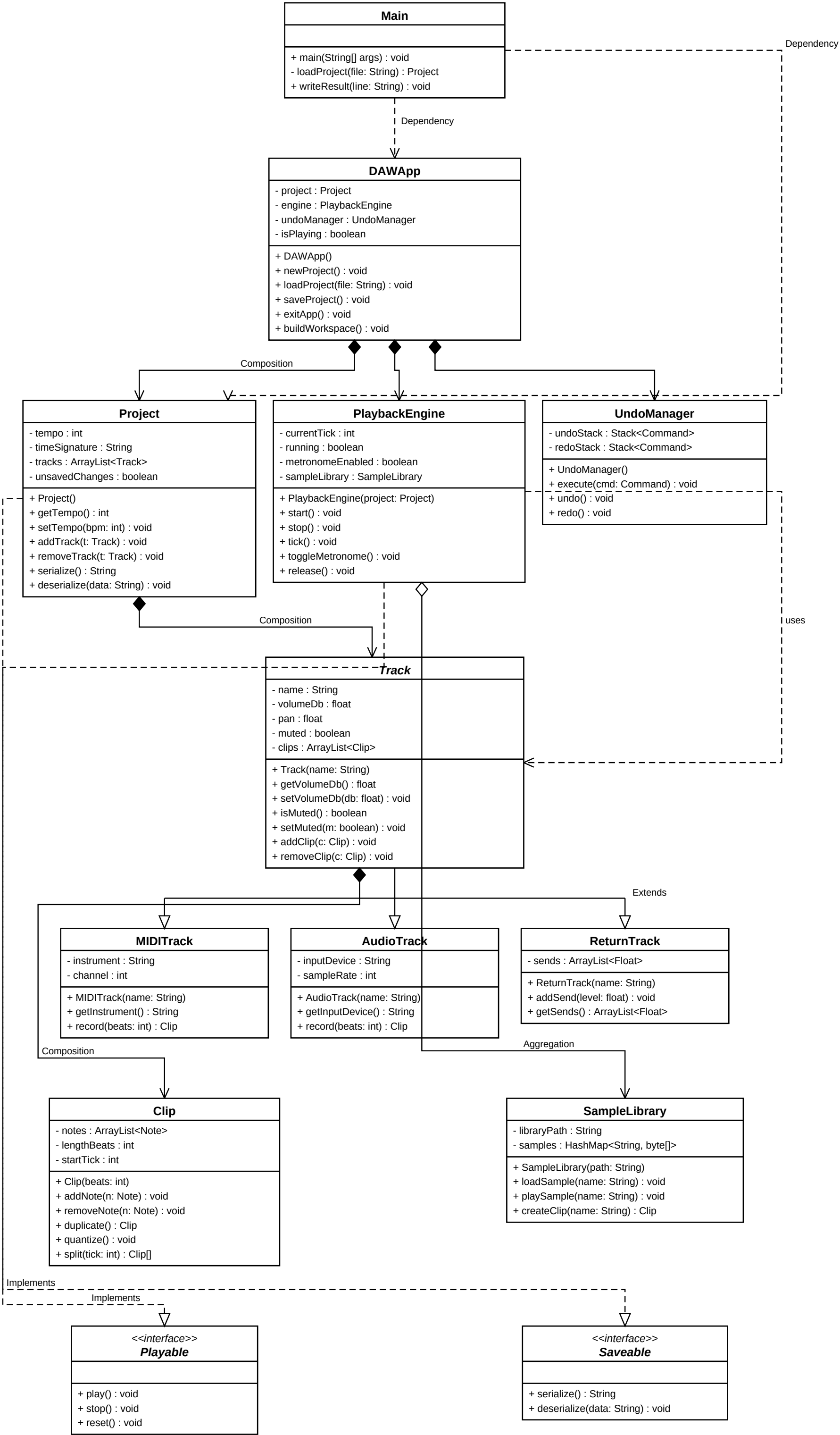
DAWApp – UML Class Diagram
