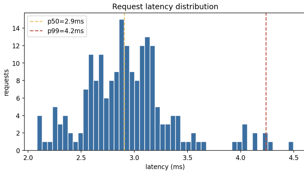
Figure 1: Latency histogram
