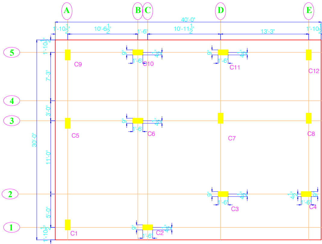
COLUMN MARKING LAYOUT.
