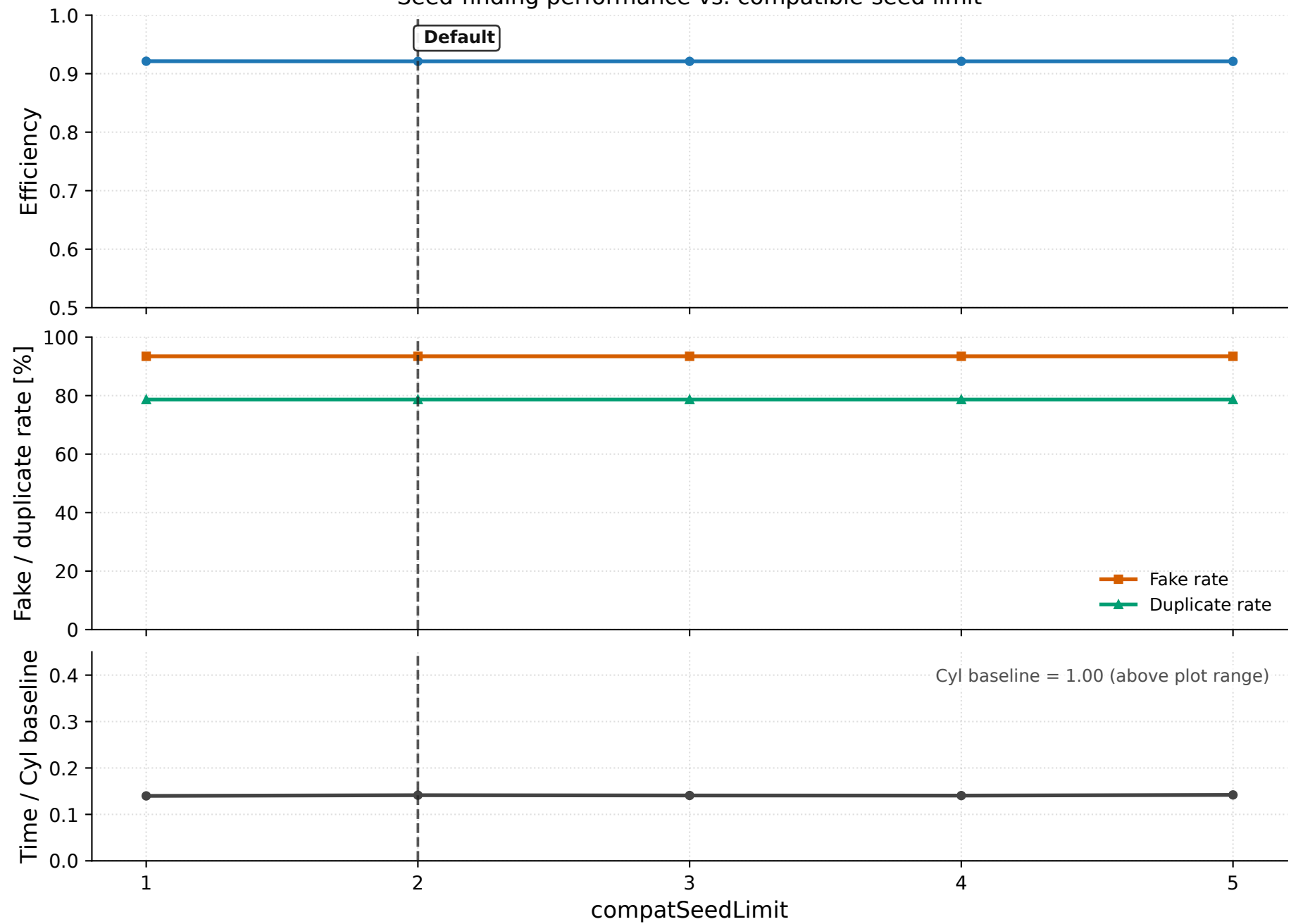
Seed-finding performance vs. compatible-seed limit
