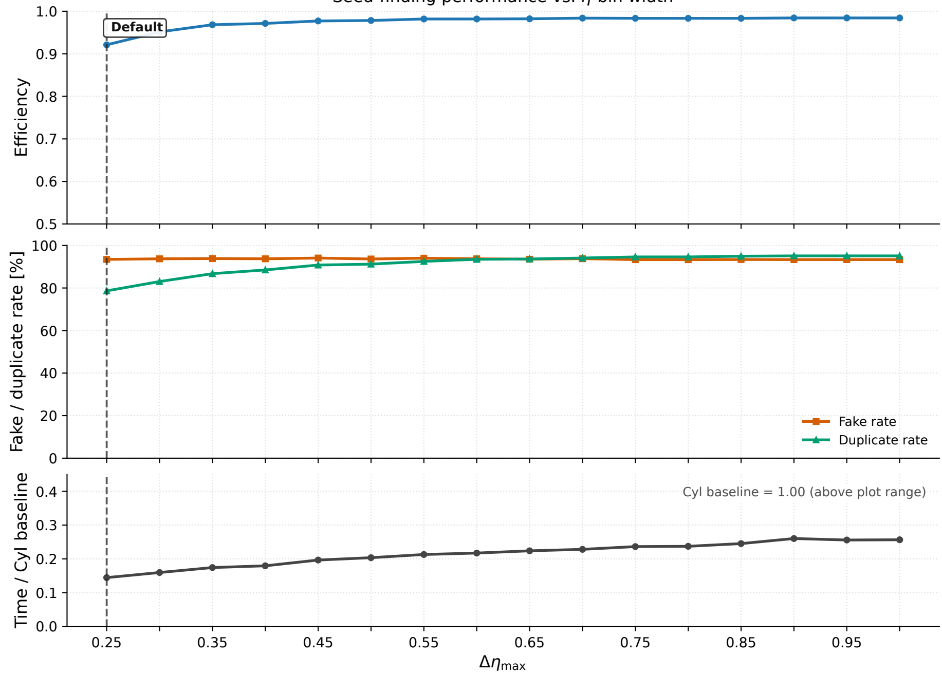
Seed-finding performance vs. \eta -bin width
