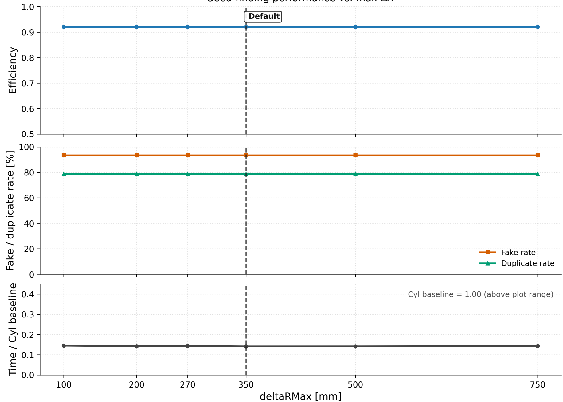
Seed-finding performance vs. max \Delta R
