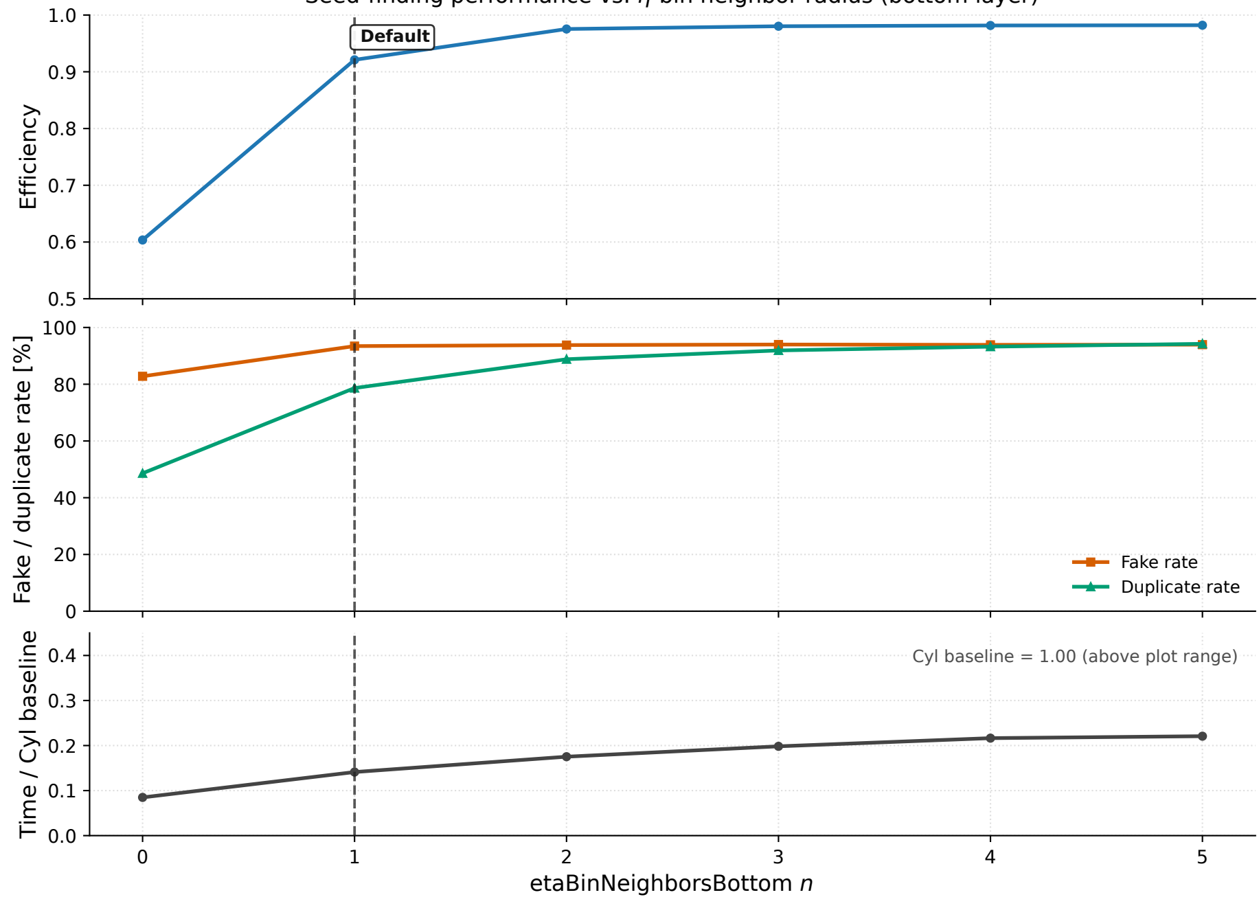
Seed-finding performance vs. \eta -bin neighbor radius (bottom layer)
