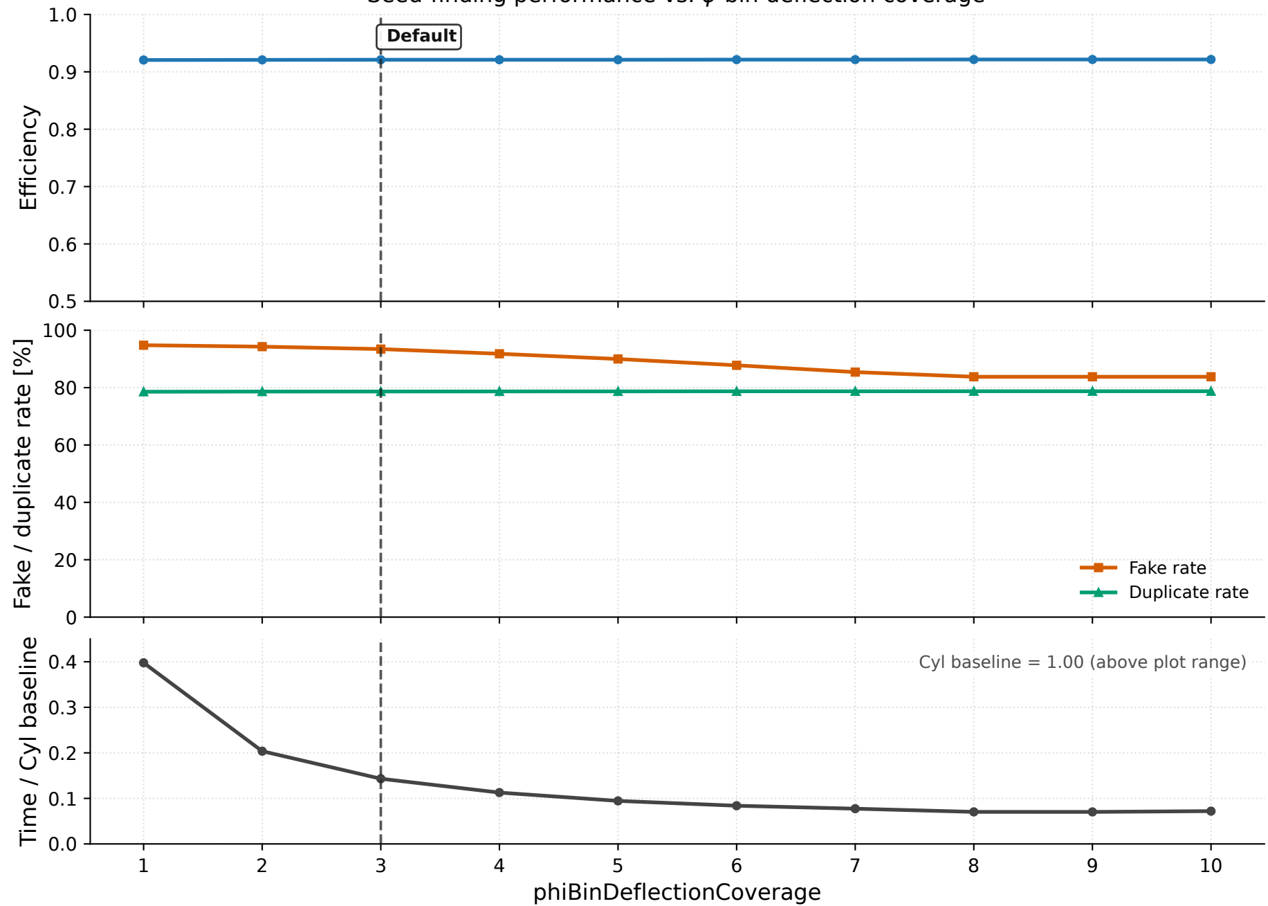
Seed-finding performance vs. \phi -bin deflection coverage
