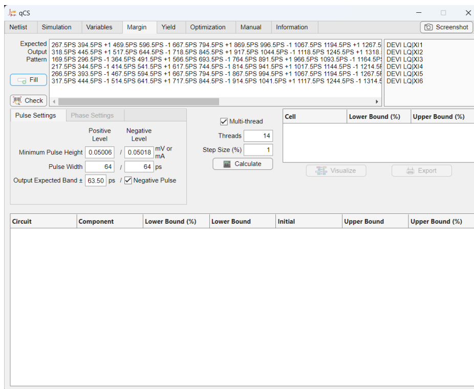
Figure 35: Margin tab after providing the specifications (AQFP).
