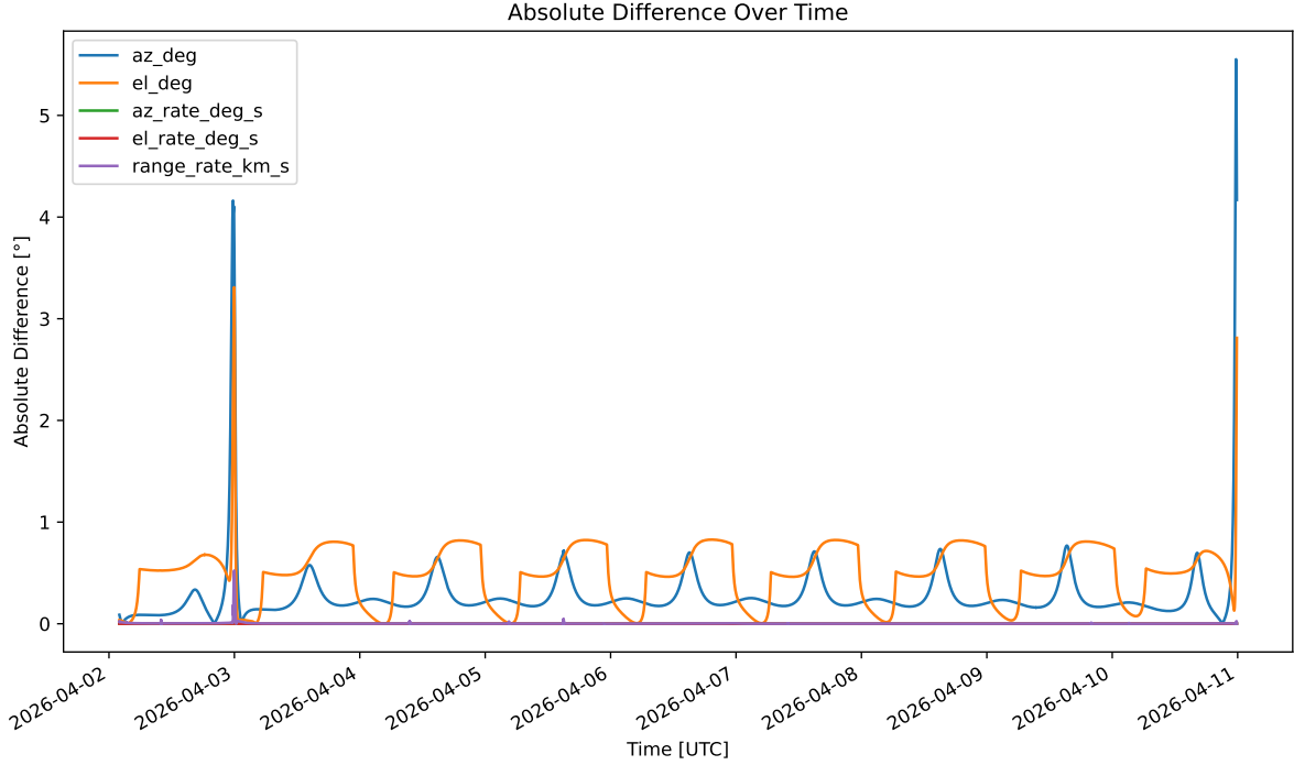
Figure 7: The difference between observer (direct) and vector data is periodic with a period of one day, indicating some systematic error.
