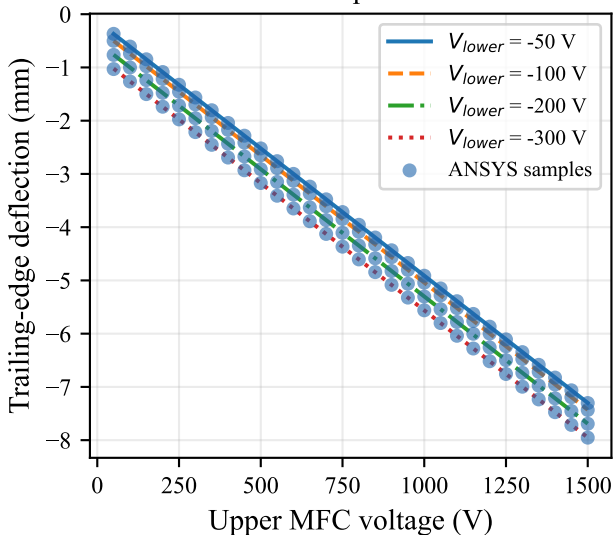
Deflection response surface
