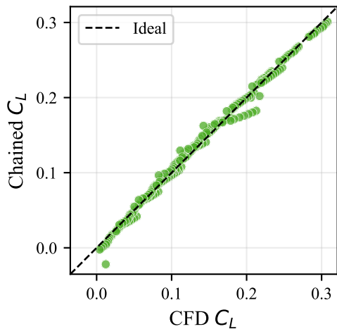
(a) Linear aero — C_L
