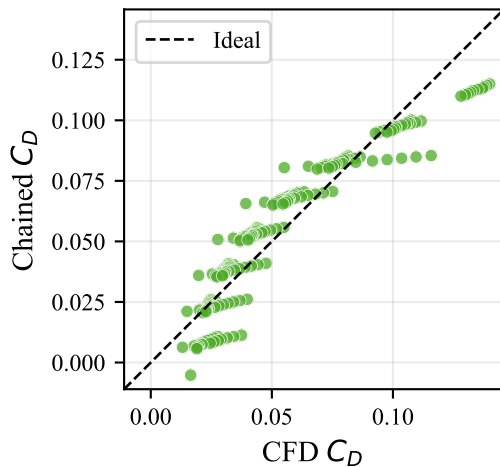
(b) Linear aero — C_D
