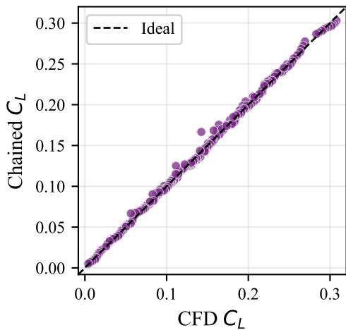
(c) MLP aero — C_L
