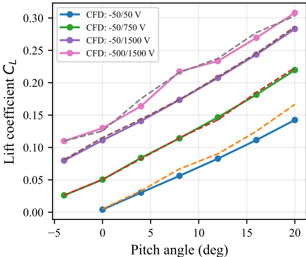
C_L vs pitch for selected voltage cases
