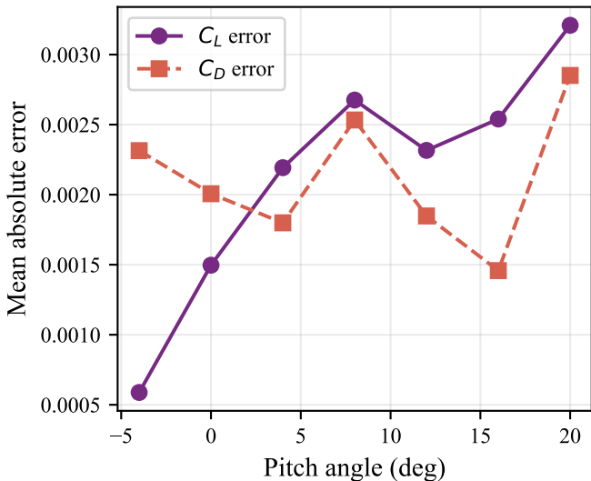
Chained model error vs pitch angle
