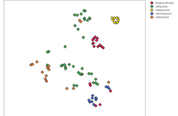
Fig. 4: t-SNE visualization for the Asian elephant dataset using the proposed method. Compared to the polar bear dataset, cluster separation is less distinct, particularly for Walking and Eating
