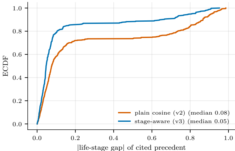
Stage relevance of citations, v2 vs v3
