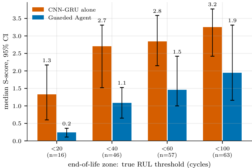
Safety penalty across zone thresholds
