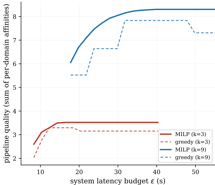
MILP vs greedy under heterogeneous specialists
