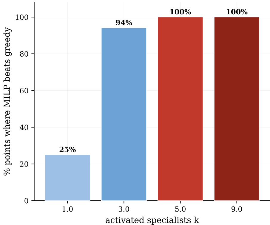
Optimization advantage grows with k
