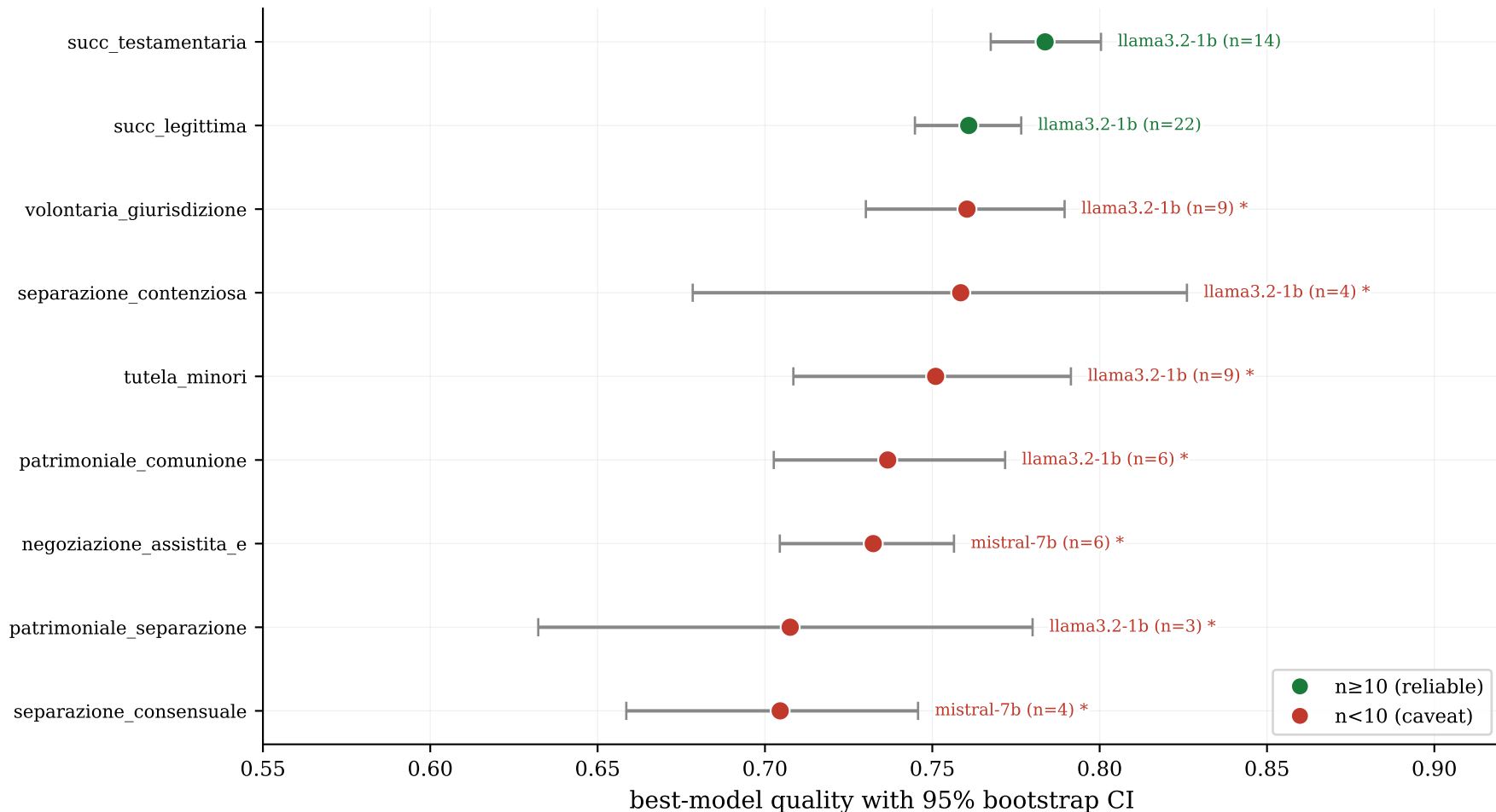
Per-domain best specialist with confidence intervals (red = n<10, unreliable)
