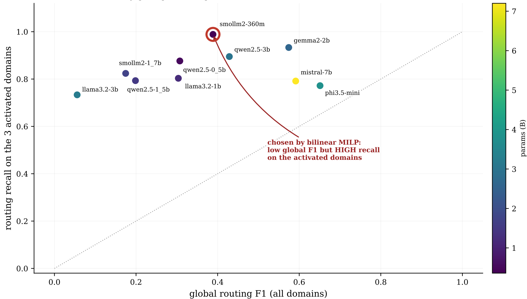
Why gating differs: global F1 is not recall on the USED domains
