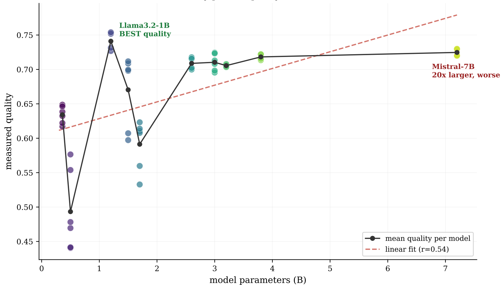
Parameters weakly predict quality ( r=0.54 ; non-monotone)
