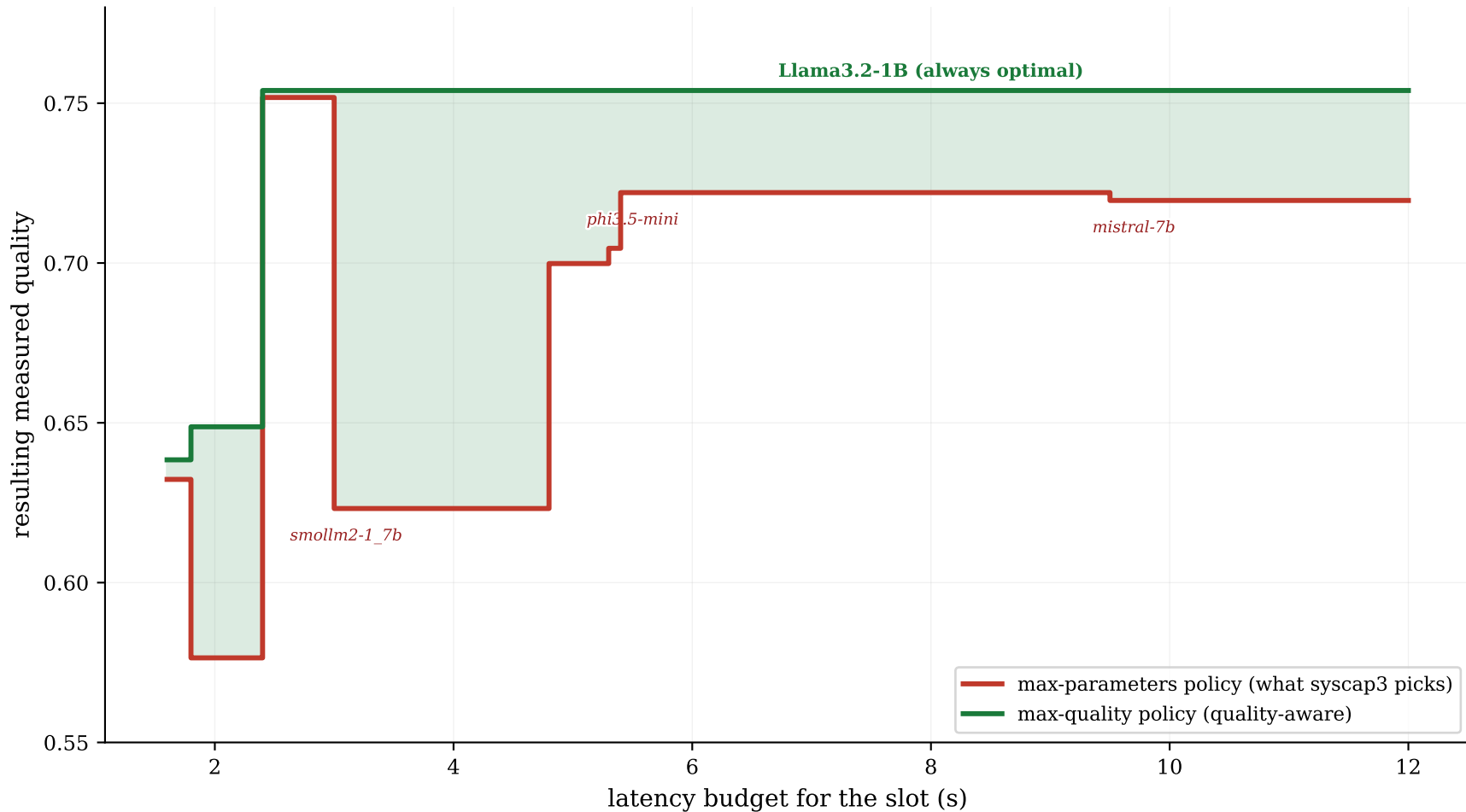
Validation: maximizing parameters wastes budget at every latency
