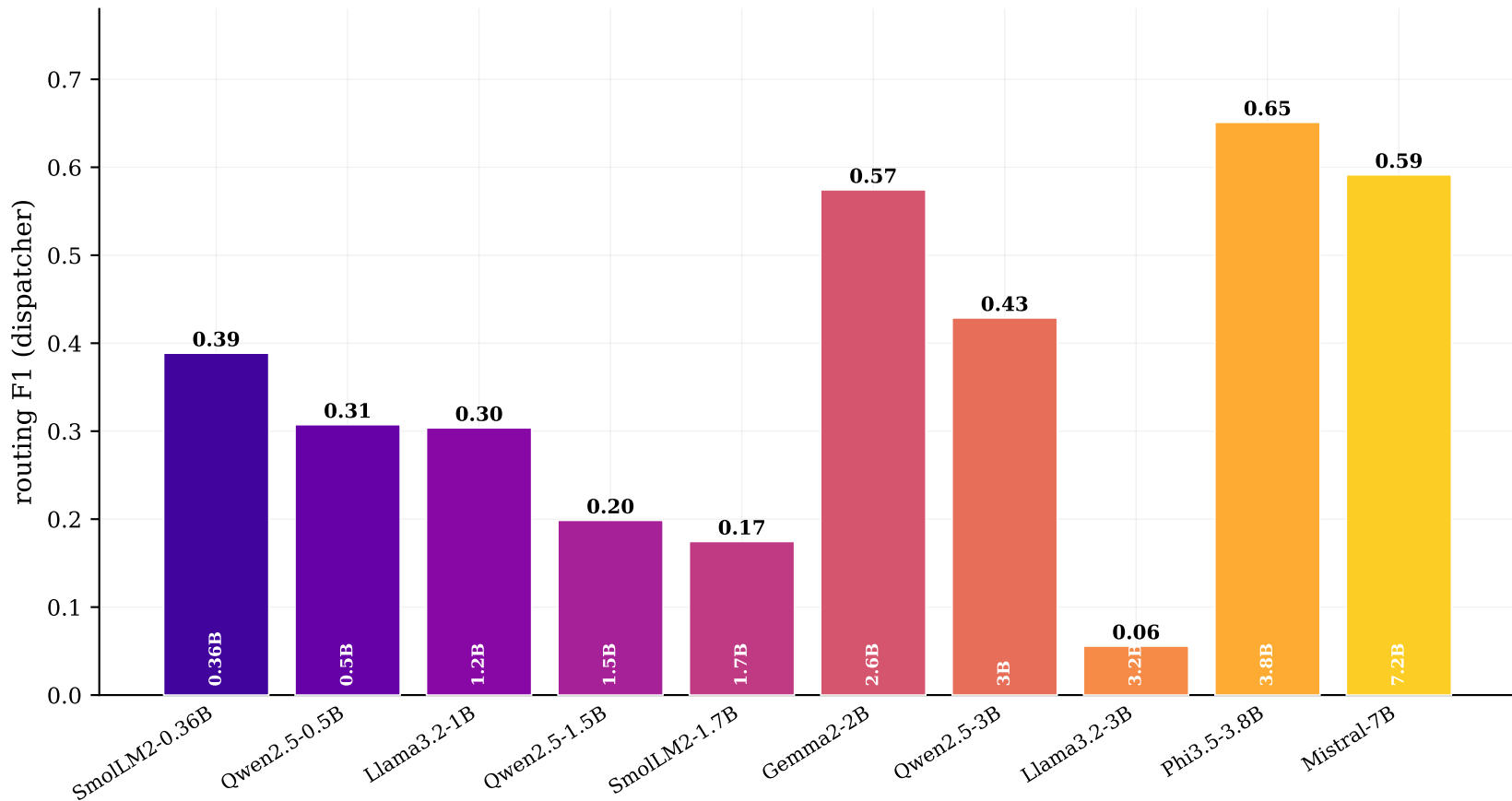
Dispatcher: routing F1 rewards LARGER models (opposite of specialists)
