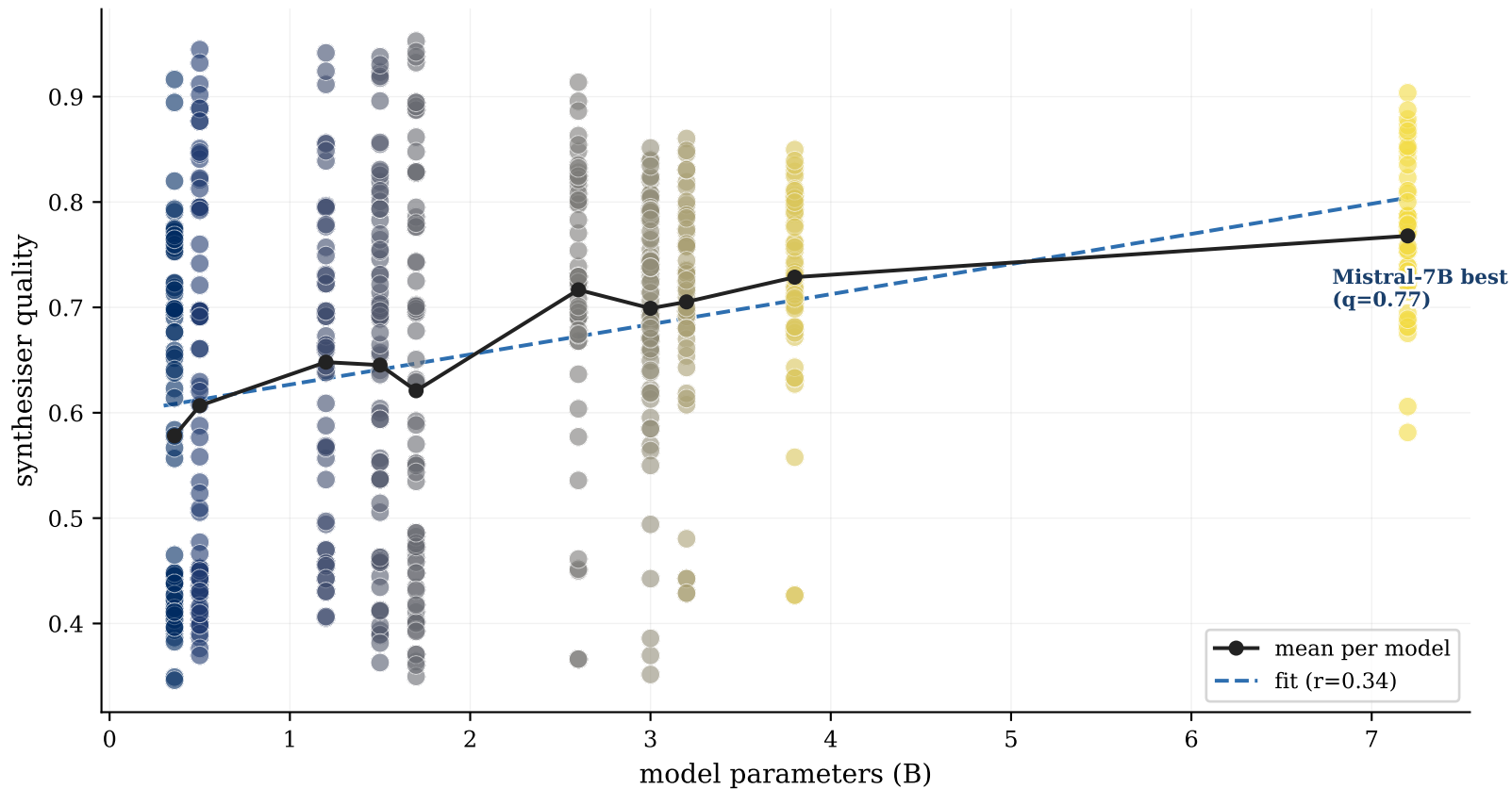
Synthesiser quality rises with size (largest model best)
