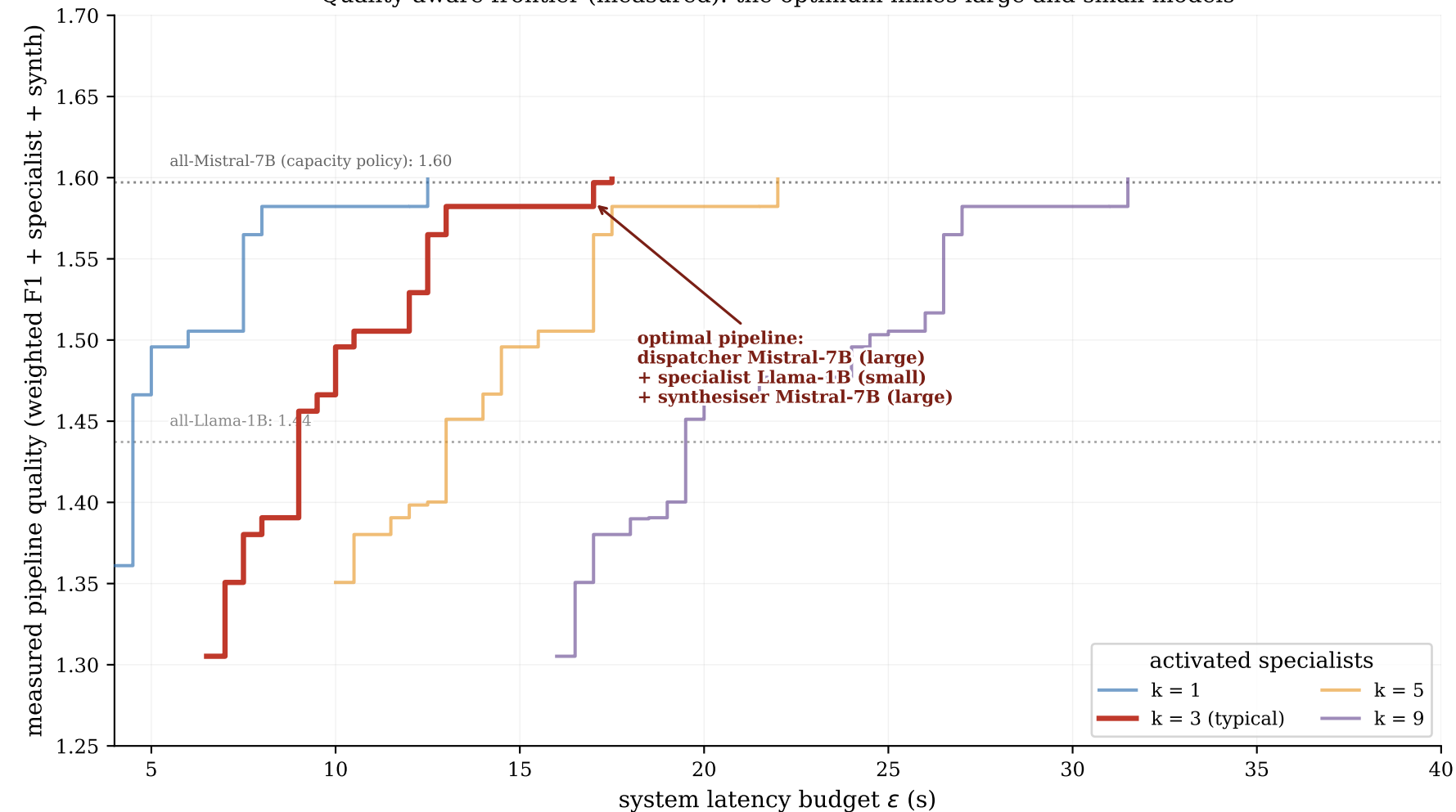
Quality-aware frontier (measured): the optimum mixes large and small models
