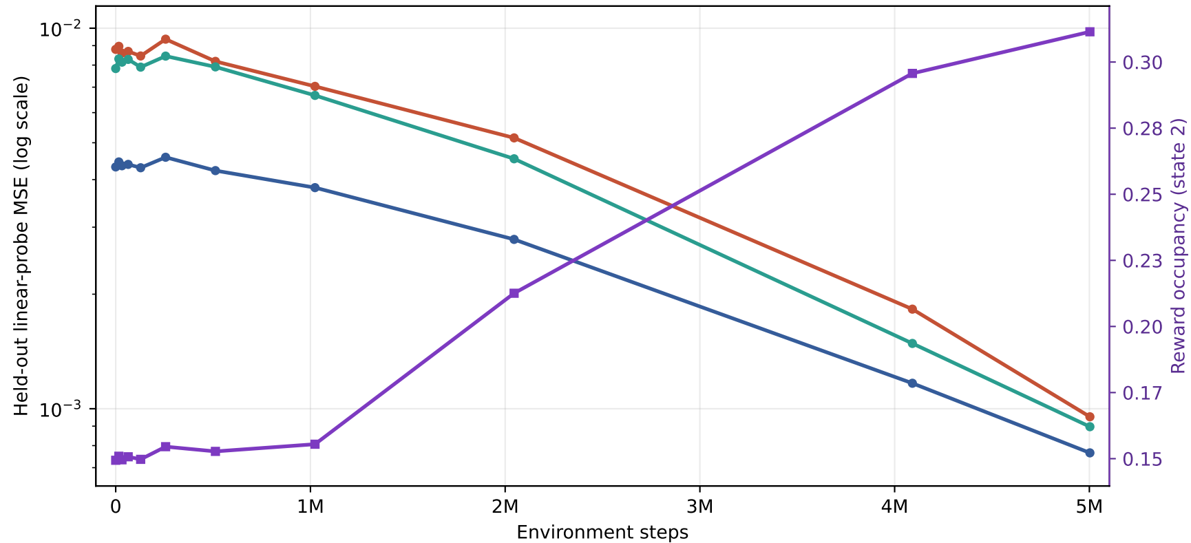
Cycle 2 SAC — reward both factors mean over seeds 42, 43, 44, 45, 46
