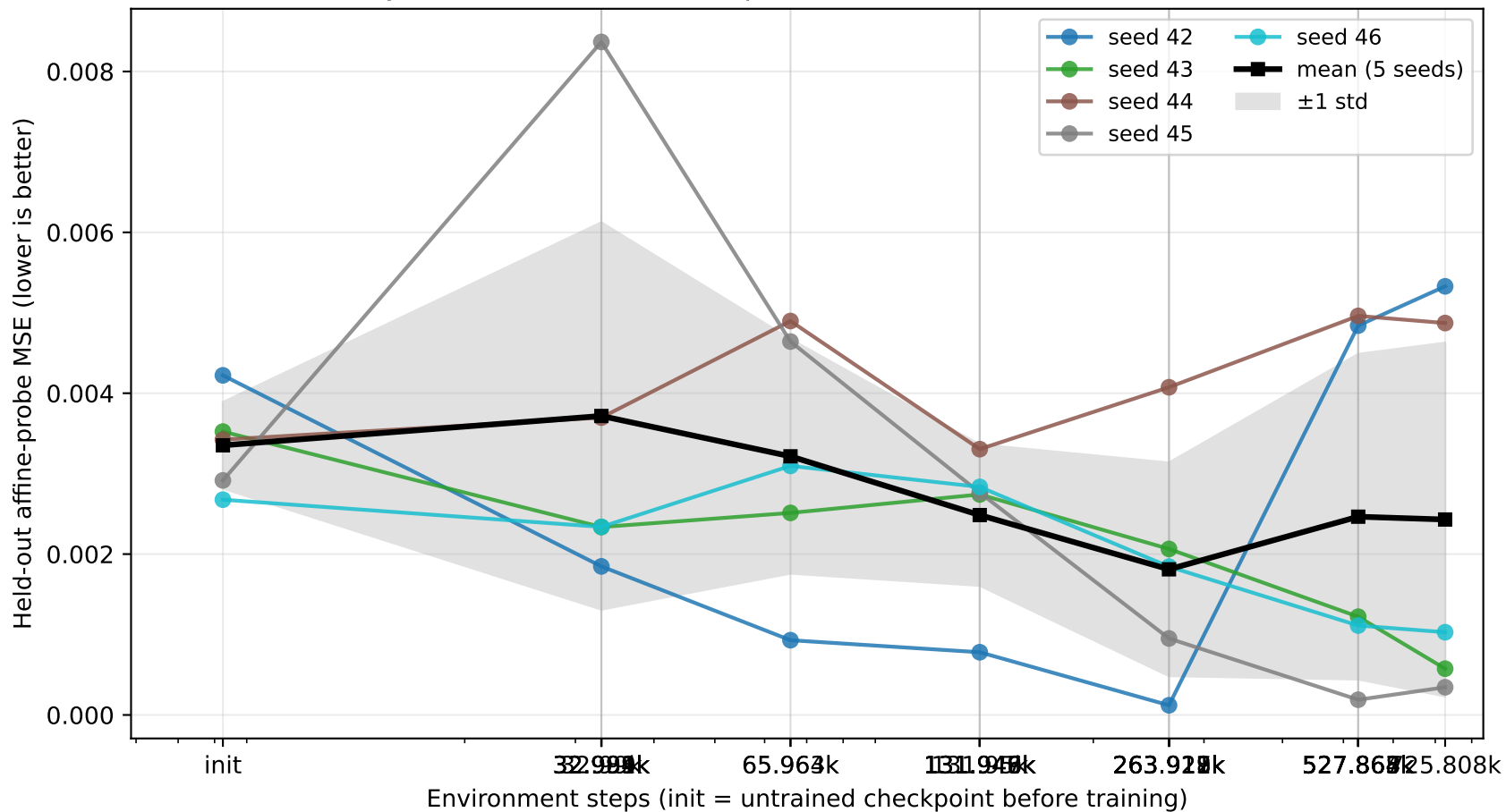
Cycle 5 variant 1 — belief probe MSE (includes untrained init)
