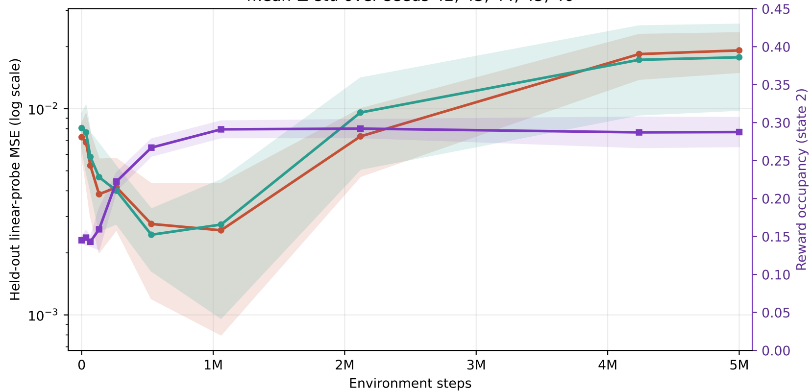
Cycle 2 PPO — reward both factors mean \pm std over seeds 42, 43, 44, 45, 46
