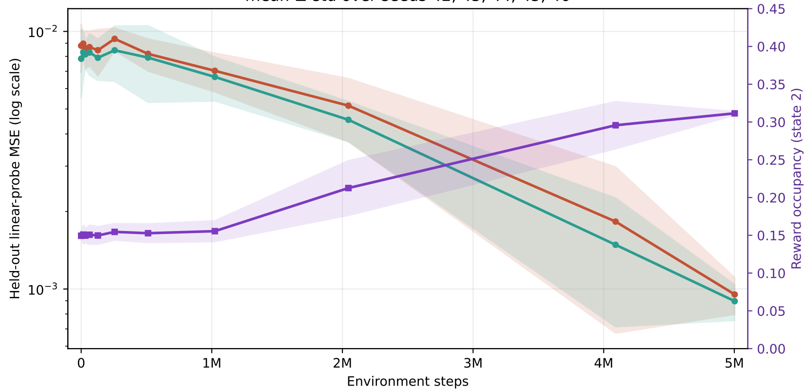
Cycle 2 SAC — reward both factors mean \pm std over seeds 42, 43, 44, 45, 46
