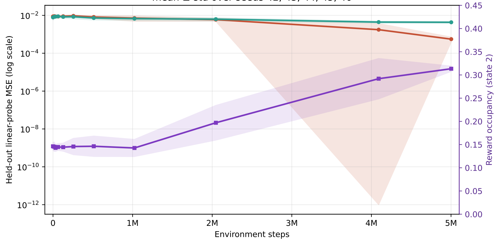
Cycle 2 SAC — reward factor 1 only mean \pm std over seeds 42, 43, 44, 45, 46
