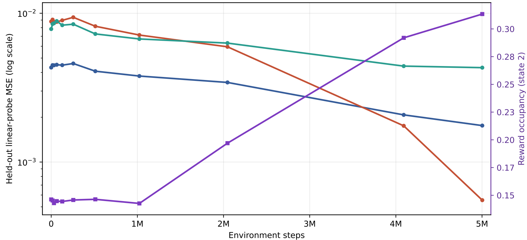
Cycle 2 SAC — reward factor 1 only mean over seeds 42, 43, 44, 45, 46
