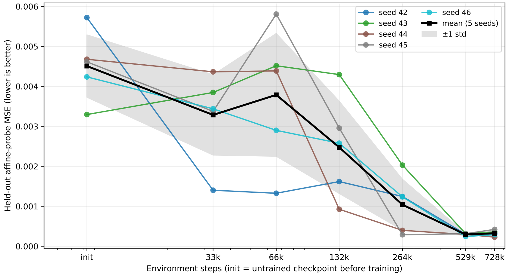
Cycle 5 variant 3 — belief probe MSE (includes untrained init)
