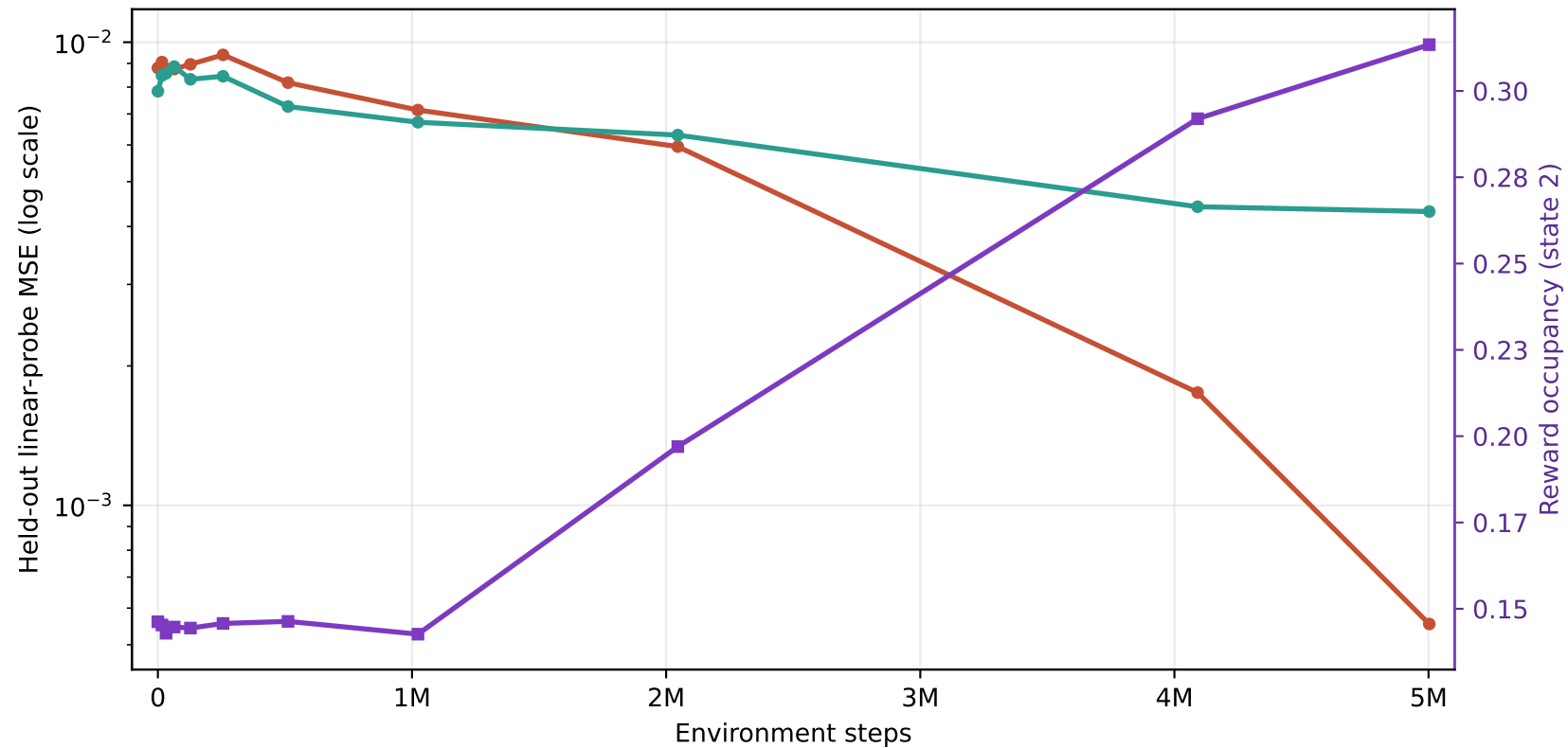
Cycle 2 SAC — reward factor 1 only mean over seeds 42, 43, 44, 45, 46
