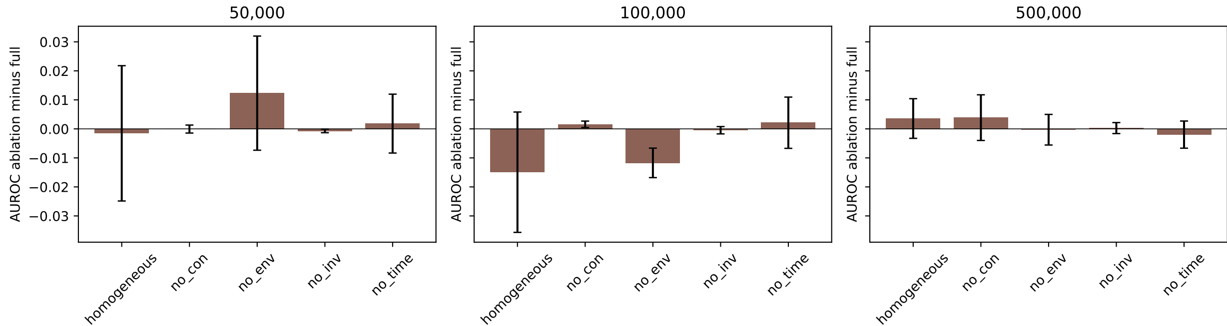
Paired ablations · mean \pm sample SD across seeds
