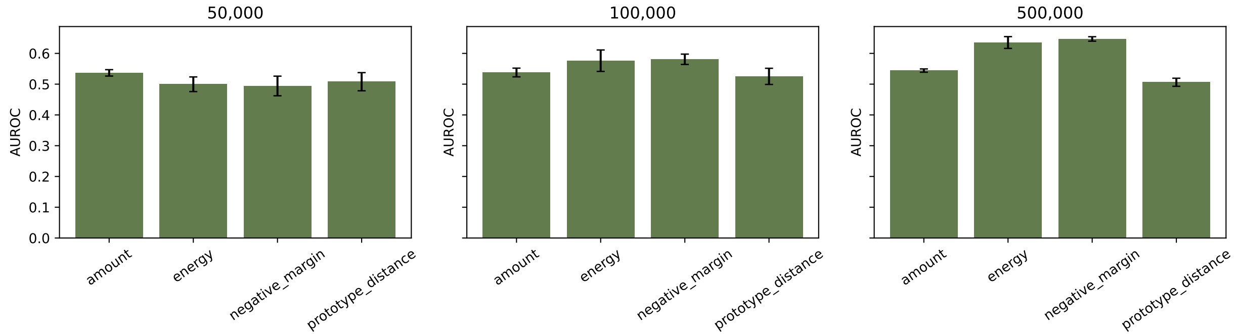
Unknown-event detection · full variant · five-seed mean \pm sample SD
